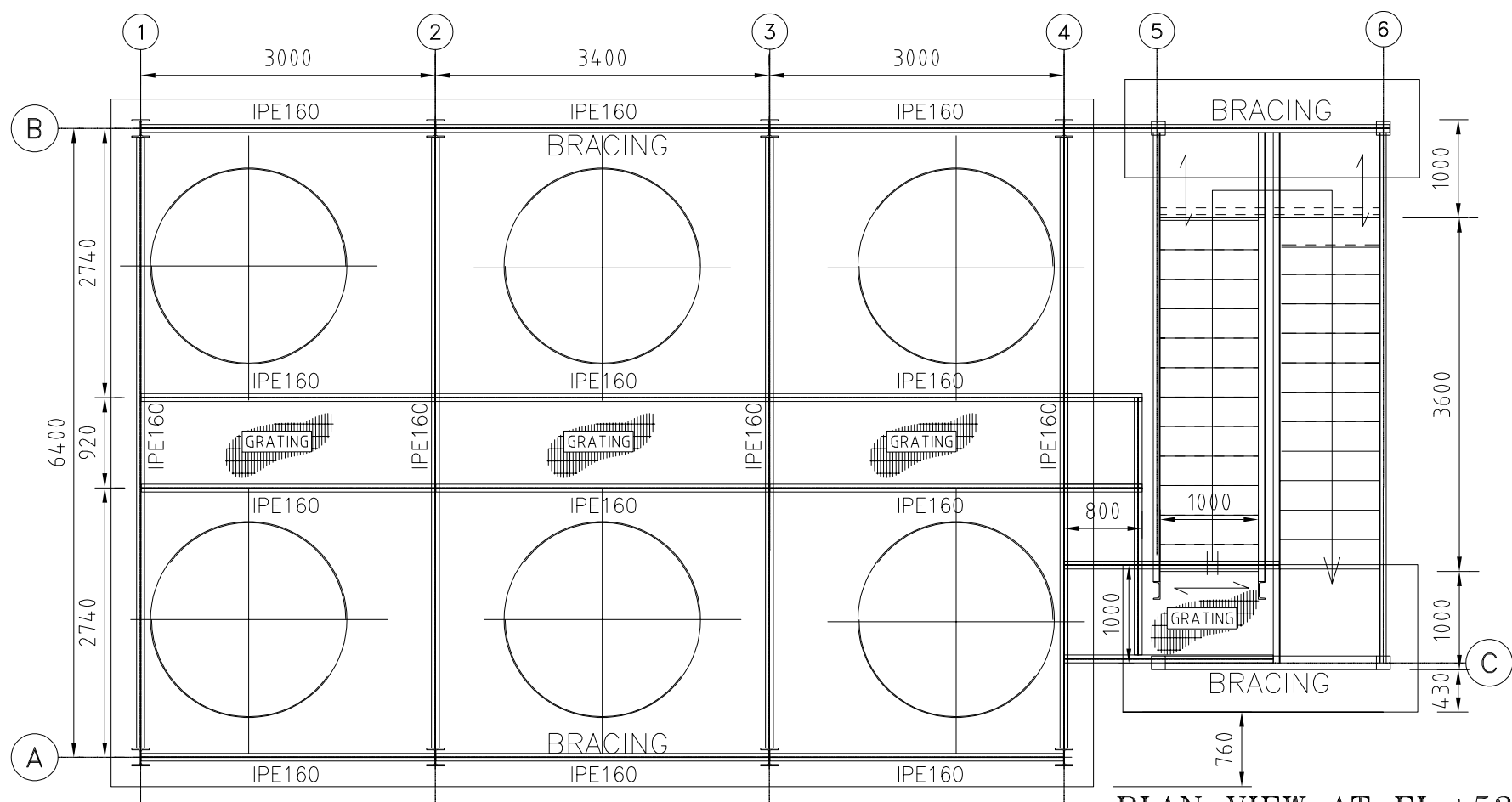
PLAN VIEW AT EL.+5300
